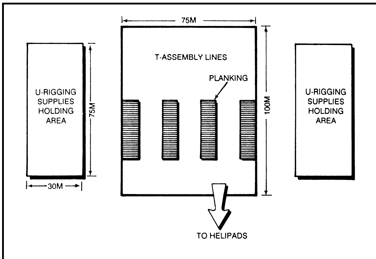
Figure 6-4. Holding areas
